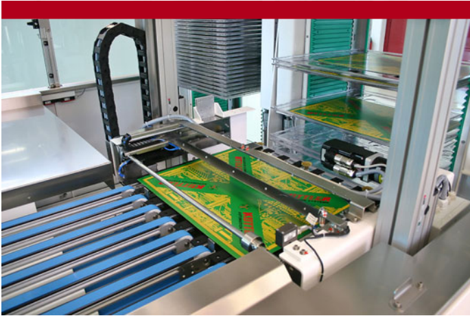
HSUE 63 with magazine exchange unit.
